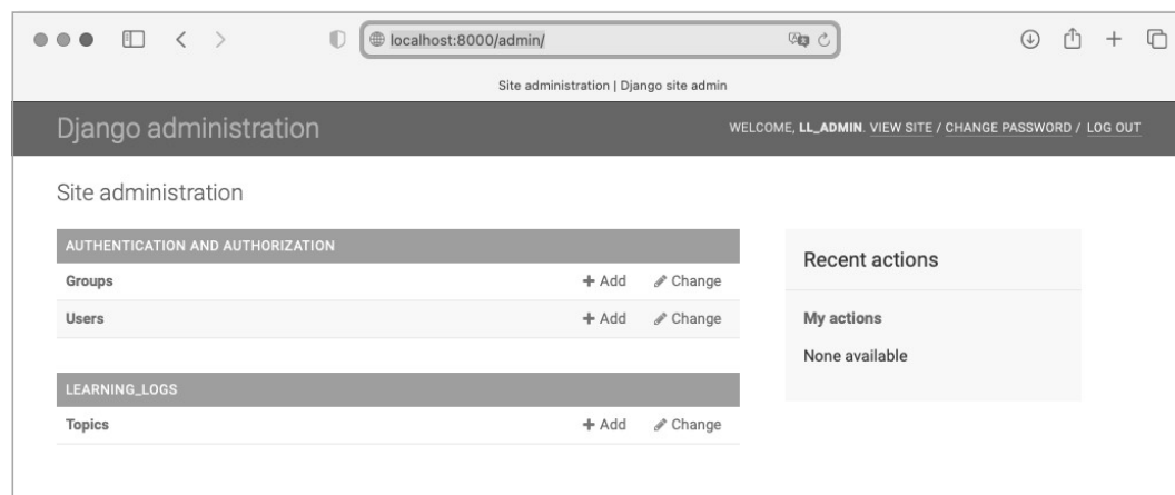
Figure 18-2: The admin site with Topic included
